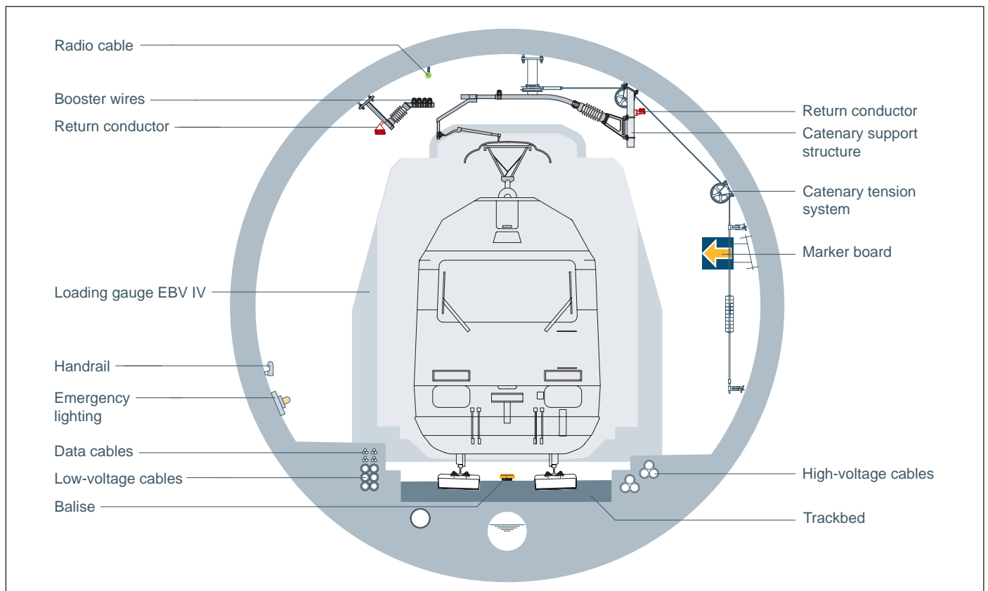
Fig 1. Each 7.76 m diameter single-track running tunnel must be equipped with low-voltage and high-voltage cables as well as telecommunications, train control and the traction power supply.
