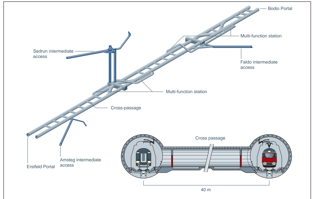
Fig 1. The Base Tunnel consists of two single-track running tunnels linked by cross-passages at 325 m intervals. 'Multi-function stations' with crossovers and emergency facilities are located at Faido and Sedrun.
