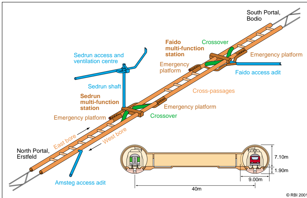
Fig 2. The multi-function stations at Sedrun and Faiedo will include crossovers between the running tunnels and emergency platforms
