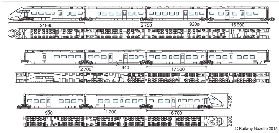
Fig 1. SBB's 11-car Giruno trainsets will have seats for over 400 passengers.
