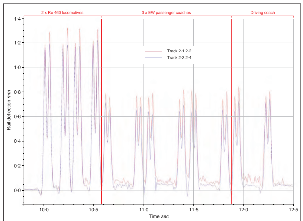
Below: Fig 3. Sequence of rail deflections recorded at 220 km/h during tests in the Gotthard Base Tunnel.
