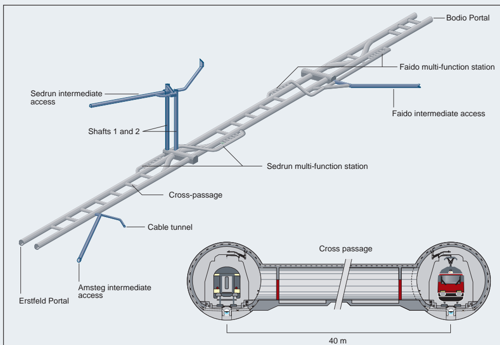
Fig 1. The Gotthard Base Tunnel is divided into three roughly equal sections by two multi-function stations where trains can switch from one bore to the other.
