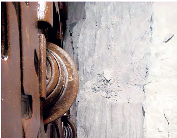
The cutting edge. Despite fears that unstable rock in the Piora zone would present a serious obstacle, the TBM passed through without major problems.
