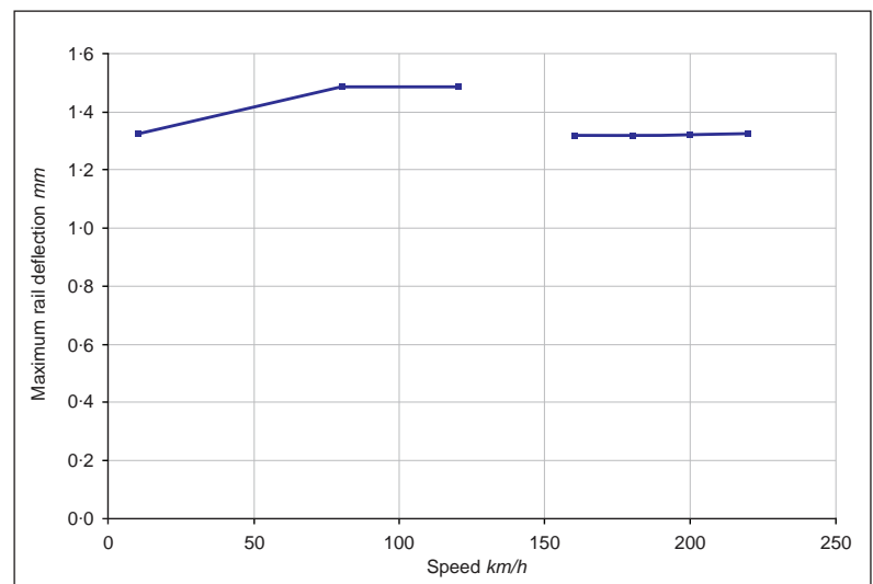
Fig 4. Average value of maximum rail deflection under locomotive axles at different speeds.
