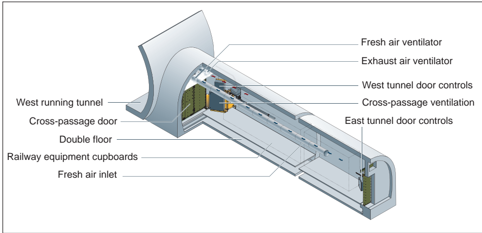
Fig 1. Cross-passages between the running tunnels are designed to be used as emergency walkways for passengers.
